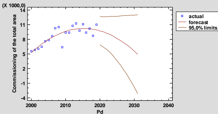
Time Sequence Plot for Commissioning of the total area Quadratic trend = 4546,57 + 697,034 t - 21,4218 t^2
